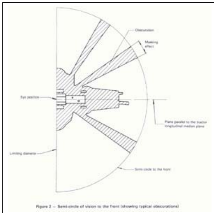
Figure 1: Semi-circle of vision to the front Source: ISO 5721, 1989, S 5
